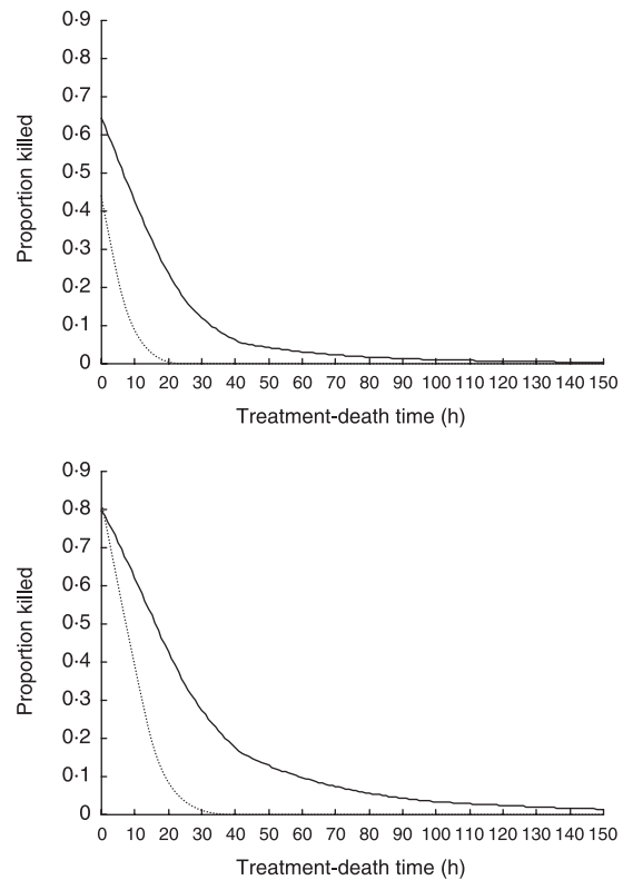
Fig. 3. Proportion of Gyps bengalensis estimated to be killed by diclofenac in relation to time between administration of the final injection of a course of the drug and the death of the treated cow (see text). Results are shown separately for a dose–response model fitted to all data from the experiments of Oaks et al. (2004) (solid line) and after excluding an outlier (dotted line). The upper panel shows results from experiment 1 with Bos indicus and the lower panel shows results from experiment 2 with young Bos taurus .
