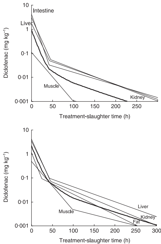
Fig. 2. Concentration of diclofenac in various cattle tissues in relation to the time between administration of the final injection of a course of the drug and slaughter. Models are the same as those presented in Fig. 1. The thin lines on each panel represent results for different tissues. The thick line shows the estimated diclofenac concentration averaged over all parts of a carcass that are available to vultures (see text). The upper panel shows results from experiment 1 with Bos indicus and the lower panel shows results from experiment 2 with young Bos taurus .
